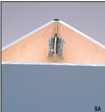
Fig. 9A & 9B Type 1R & 1L Latches and slot Receivers to fabricate polygonal structures, kiosks, etc of 3 or more panels. (See TDSs 17 & 28)
